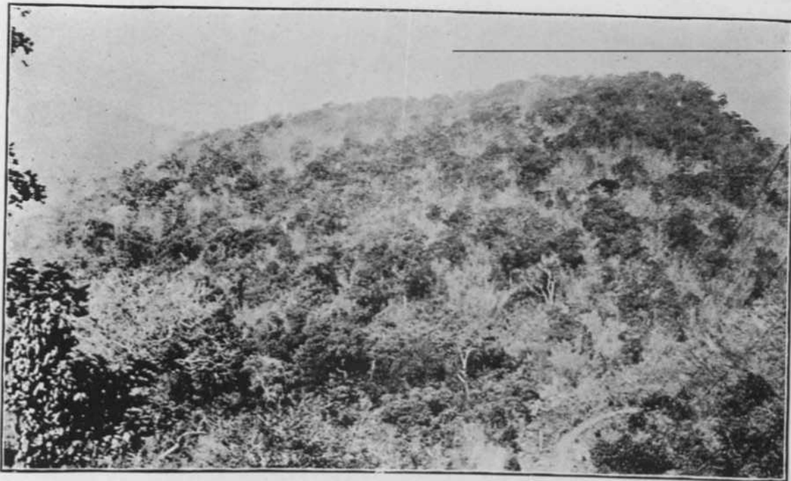
Fig. 1. Ml. Oak Forest. General view showing the open character (with grass Wank*) of it. n^L n, of the «0-100- 3,000'. TSM? Iron V" "(•» T e ^ S? Su&hiJSS Sand*Ma, (TEocene). Season: late April (1924). Elevation: about 1100: L. Dudley Stamp.
