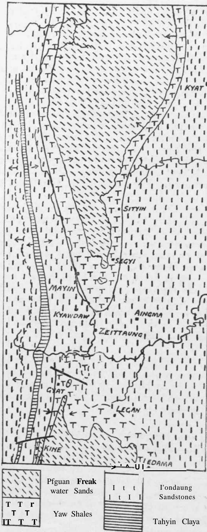
Fig. 7. Geological map of part of the Lower Cliindwin District. Scale 5 mil«s=1 inch. L. D. S.
