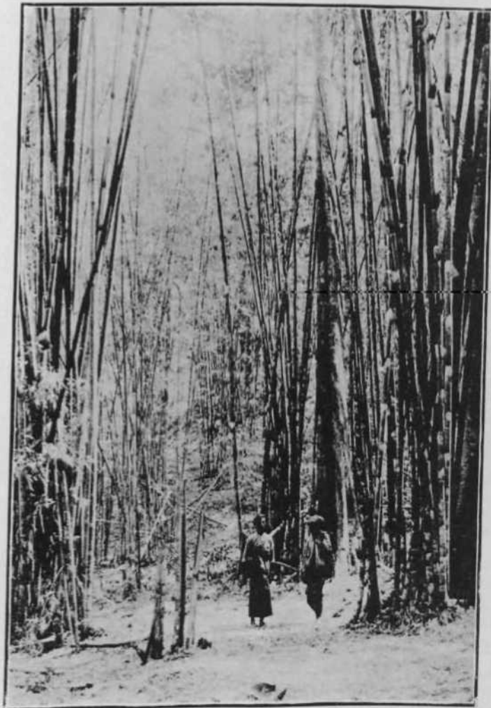
Fig. 2. L4c. Bamboo (Kyilhaup. Bambusa potyiorophii ) in Moist Touk Forest. Rainfall: about 70". Geology: Alluvial fine sandstone. Season: March 1924. 1 mile East of Ngalawa Bungay. Tharrawaddy Division. Photo: L. Dudley Stamp.
