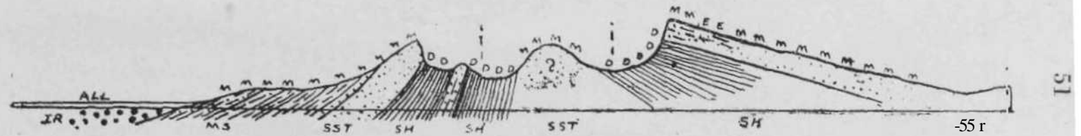
Fig. 11. Geological and Vegetations! section across the western side of the Pegu Yoma. Geological:—all=alluvium. Ir=Irruadilimi. remainder is Pt-puan comprising MS (mixed sandstones and shales), Sst (sandstone), Sh (shales). Vegetation:— M=Moiit Teak ;iml Pyinkado Forests; li^Drj Teak Forests; R- nfn Trfrfm. Notice the Dry Teak Forest on the infertile shale belts.
