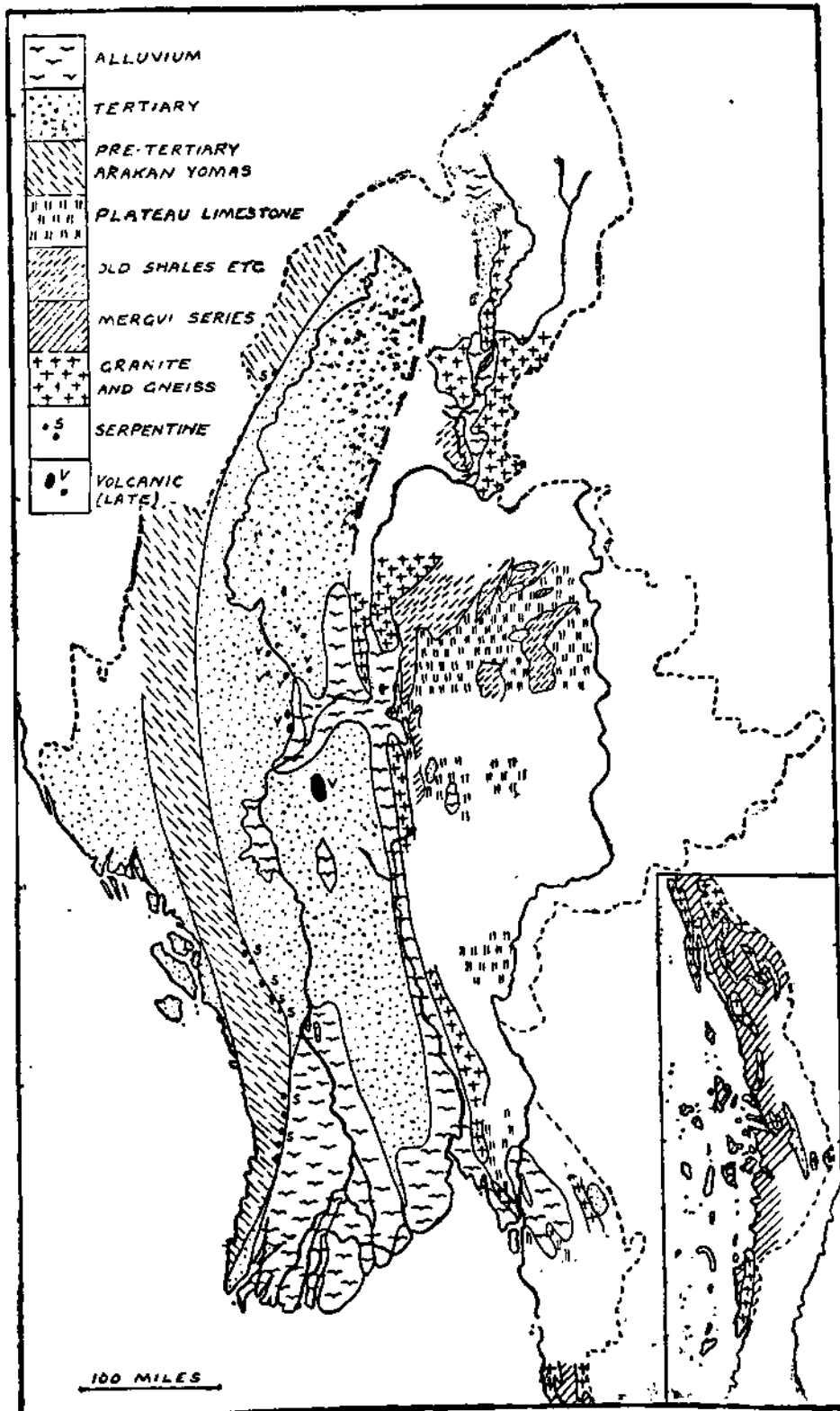
FIG. 1. A geological Sketch map of Burma, reduced from the maps published by the Geological Survey of India. The blank areas have not been mapped geologically but consist mainly of old rocks, with limestone predominating.
