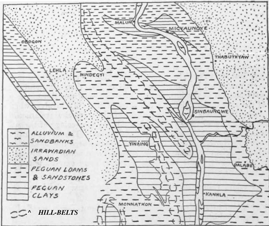
Fig. 5. Geological map of part of the Irrawaddy Valley within the borders of the Dry Belt. Scale 1 inch = 10 miles. L. D. S.
