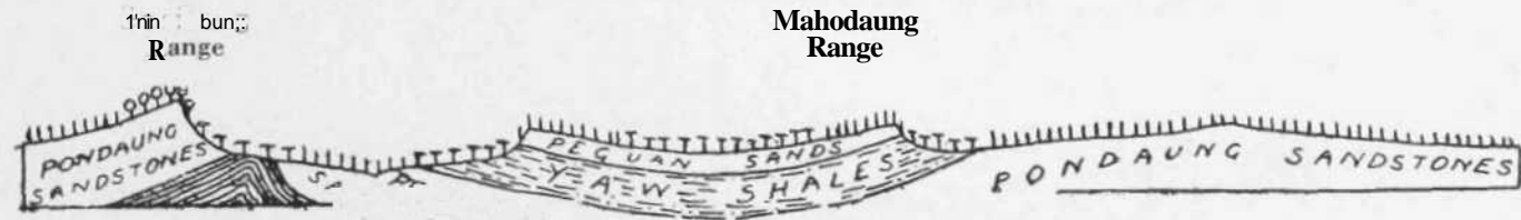
Fig. 9. Geological and Vegetations! section across the maps aho\wi in Figs. 5 and 6. I=Indaing; T=Teak Forest. For explanation see text. /.. U. S.
